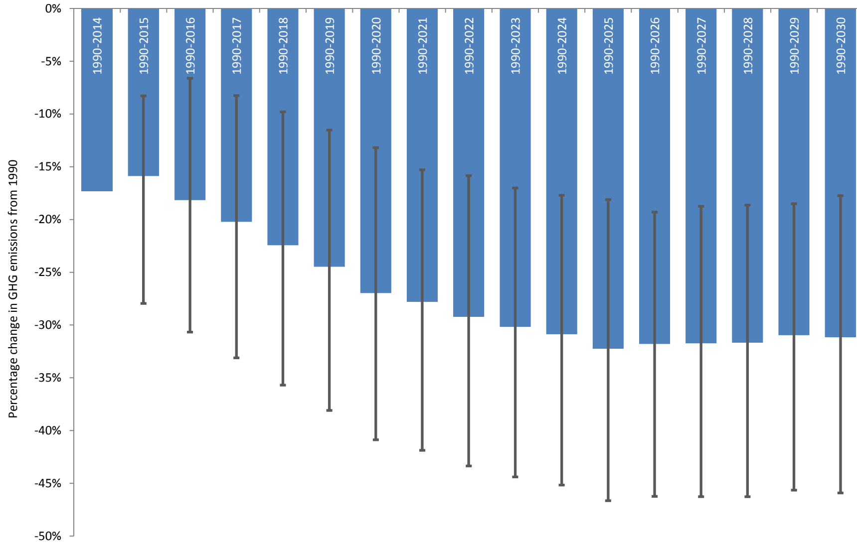
Figure 1 - Percentage change in NI Greenhouse Gas (GHG) emissions 1990-2014 to 1990-2030 including sensitivity analysis of higher/lower emission scenarios
