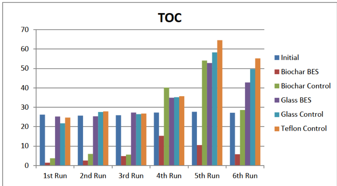
Figure 6 Total organic carbon in mg/l.
