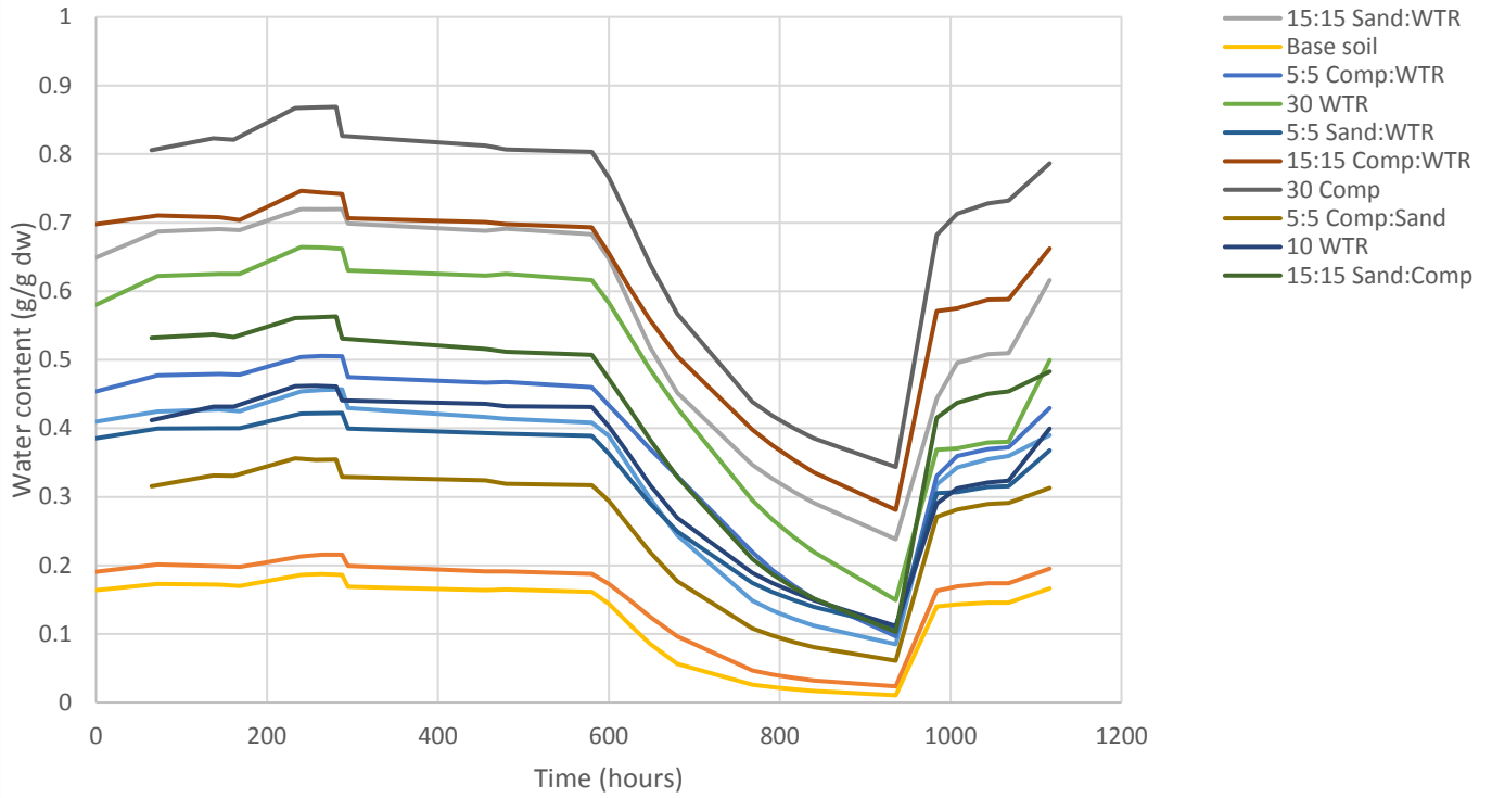
Figure 15 - Water holding capacity (g/g dw)
