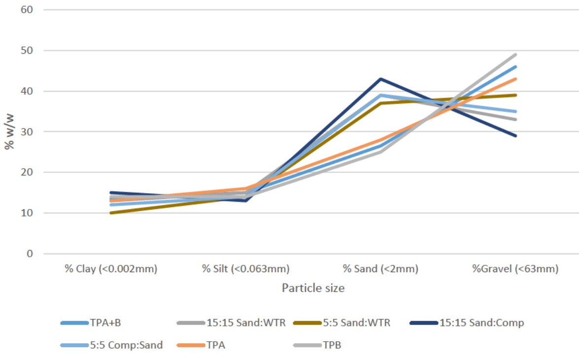
Figure 4 - Particle size distributions (Combinations with sand)
