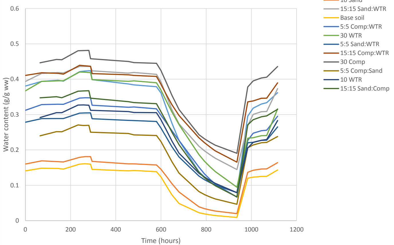
Figure 16 - Water holding capacity (g/g ww)
