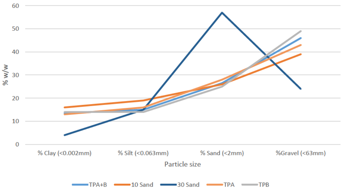
Figure 3 - Particle size distributions (Sand)
