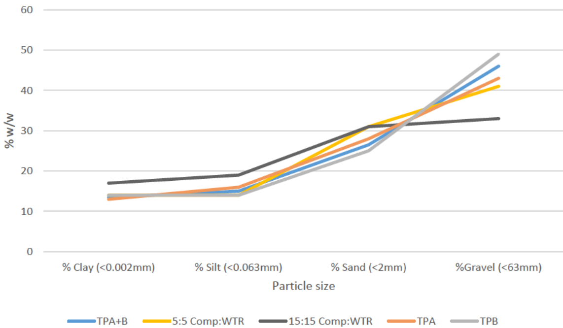
Figure 5 - Particle size distributions (Combinations of compost and WTR)
