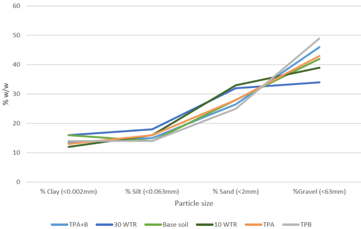
Figure 2 - Particle size distributions (WTR)
